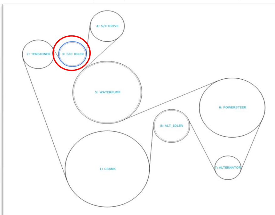
Belt route for idler system (6PK2285 with 80mm drive)
