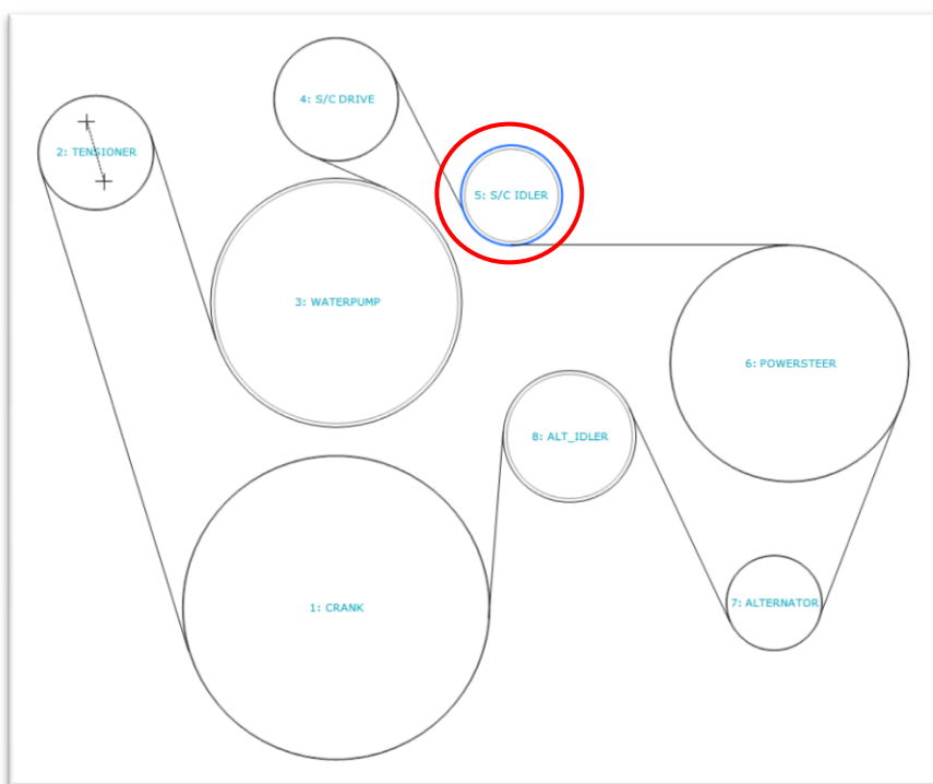
Belt route for idler system
